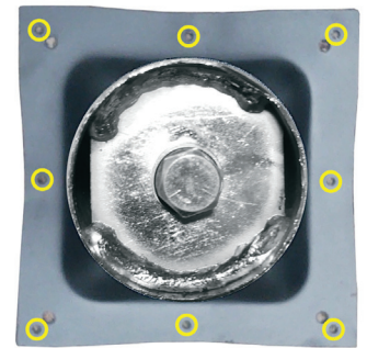
12. Use the 8 perimeter holes on the spider (circled in yellow) to fasten the base to the table top.
